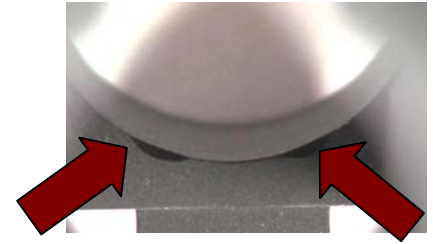
View of the feed ramps cut in the M4 receiver from the rear of the receiver. Barrel is not installed.
